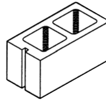
8x8x16 Sash
